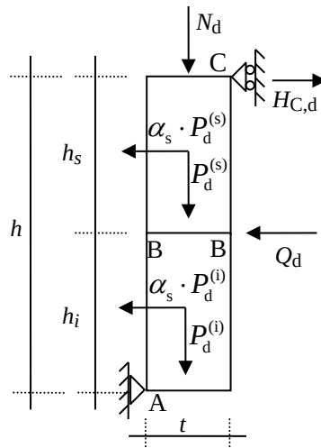
Figure 5-6 – Collapse mechanism by vertical flexure.
