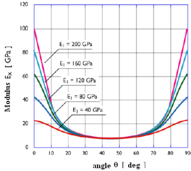
Figure 9-6 – Modulus of elasticity, E_x , as a function of \theta for balanced fabric depending upon the modulus of elasticity, E_1 ( E_2 = E_1 ; G_{12} = 3 GPa; \nu_{12} = 0.35 )
